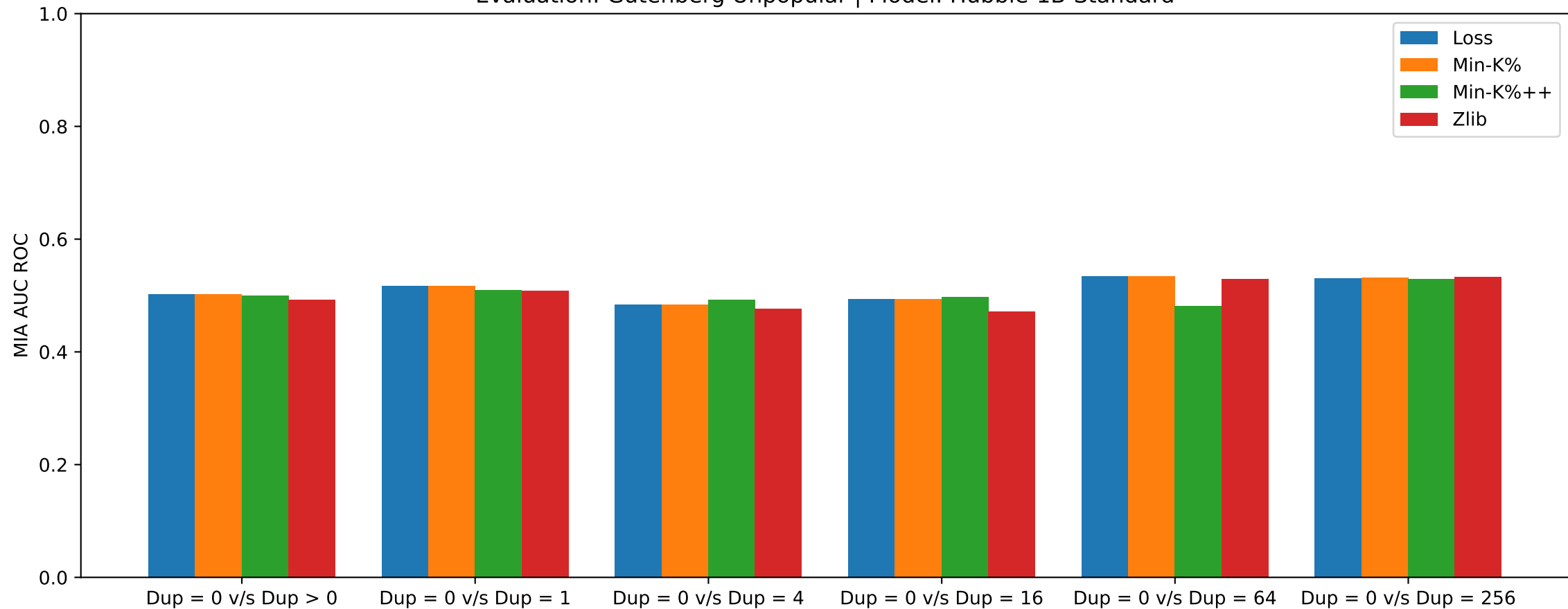
Evaluation: Gutenberg Unpopular | Model: Hubble-1B-Standard
